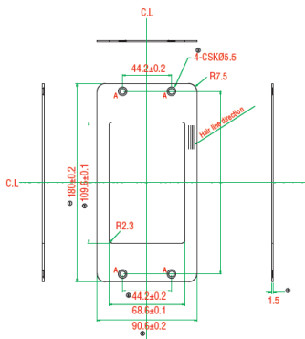
VP-FD1 (front decorative plate)
